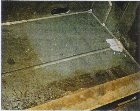
Intershield 300 in a ballast tank after 13 years in service.
